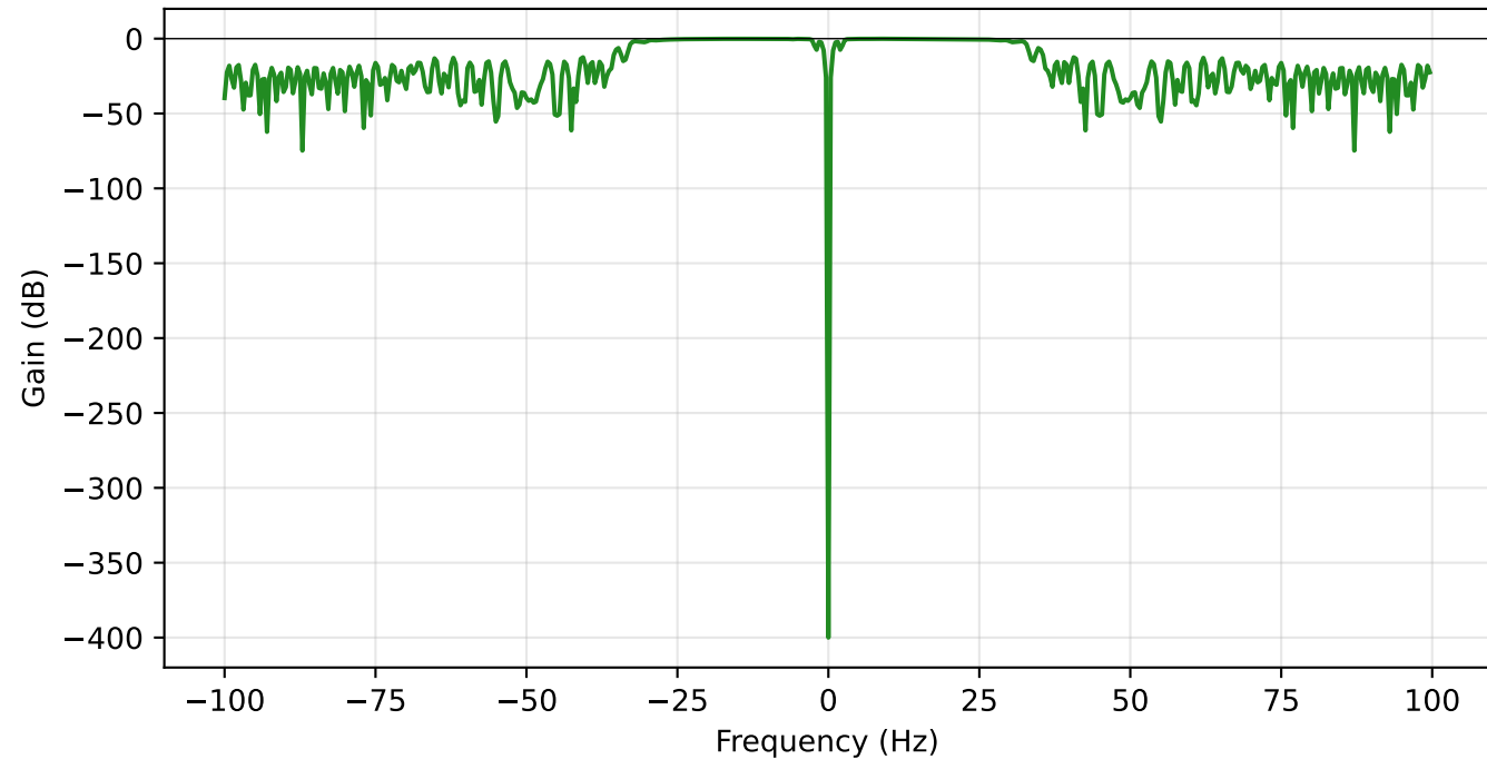
Wiener filter magnitude response |W(f)|
